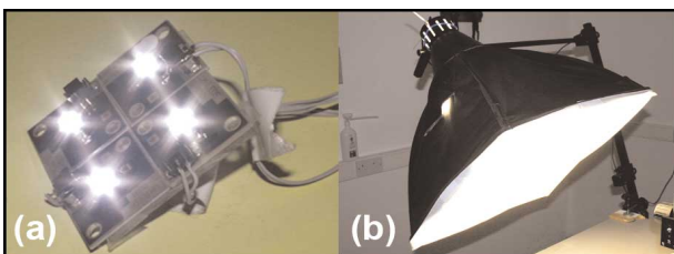
Figure 8 - a PrevARTI RLS LED array and b a commercially available “softbox”
